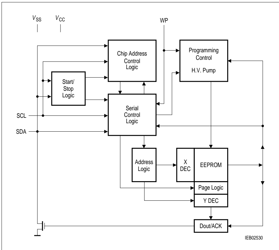
Figure 2 Block Diagram
