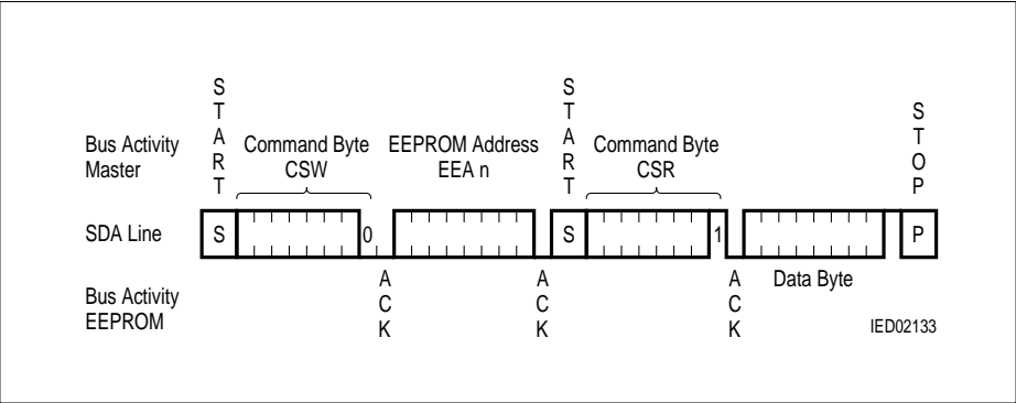
Figure 11 Random Read
