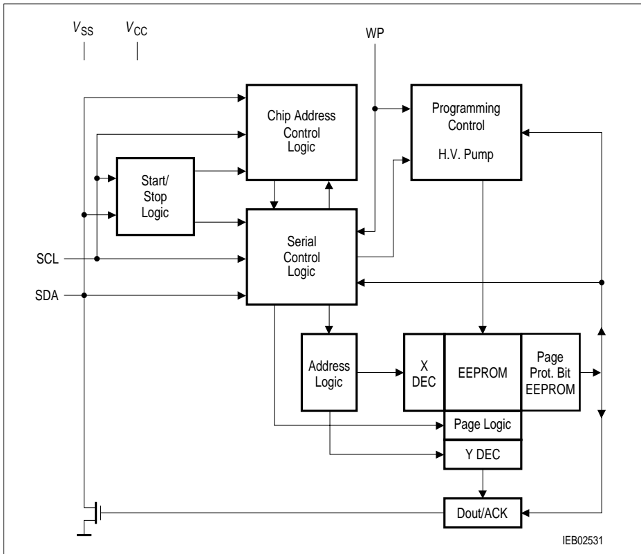
Figure 2 Block Diagram
