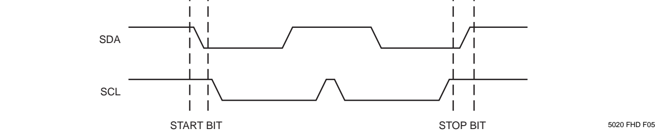
Figure 3. Start/Stop Timing
