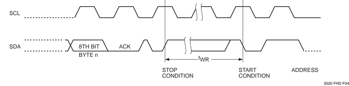
Figure 3. Start/Stop Timing
