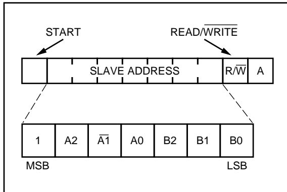
FIGURE 4-1: CONTROL BYTE ALLOCATION
