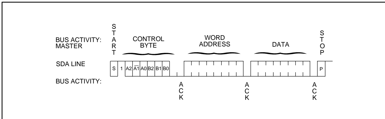
FIGURE 5-1: BYTE WRITE
