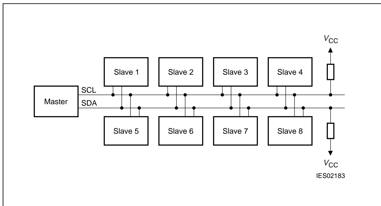
Figure 3 Bus Configuration
