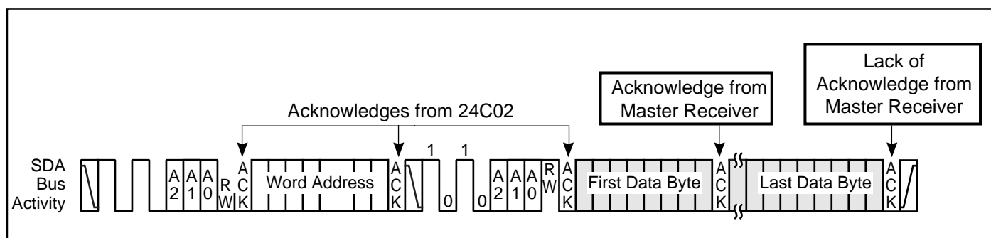
Figure 9. Sequential Read
