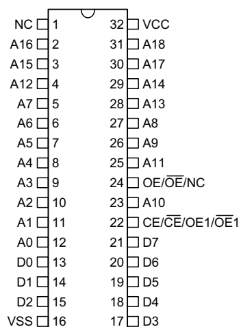
HT23C040 – 32 DIP/SOP
