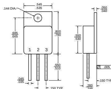
TO-254AA
