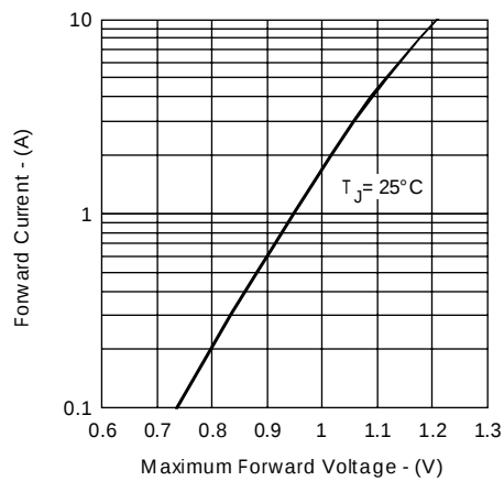
Fig. 2 - Forward Characteristic
