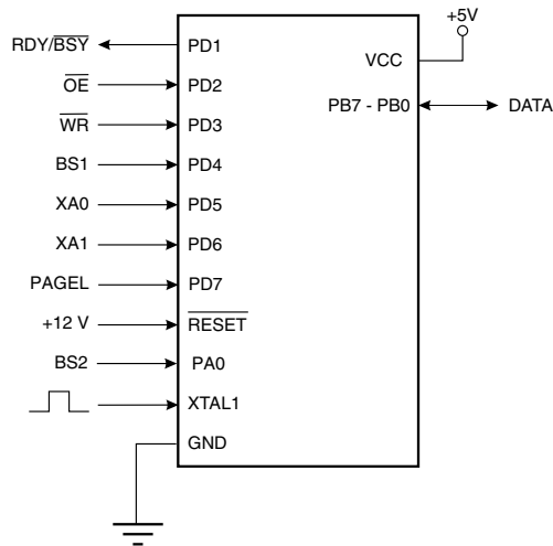
Figure 75. Parallel Programming
