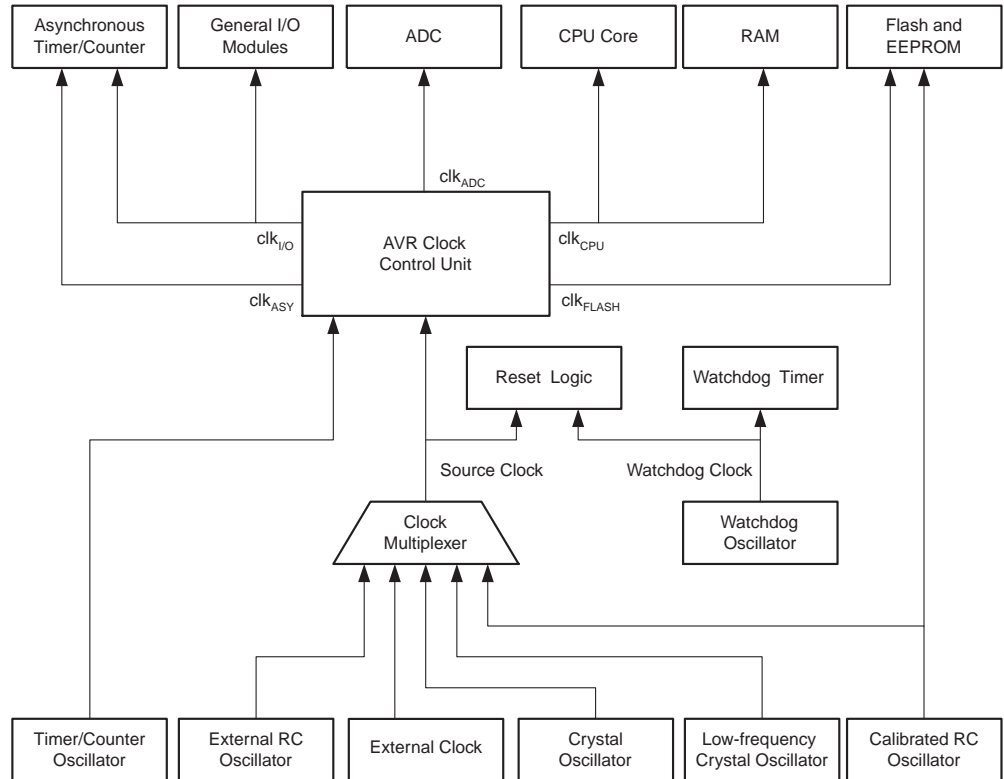
Figure 18. Clock Distribution
