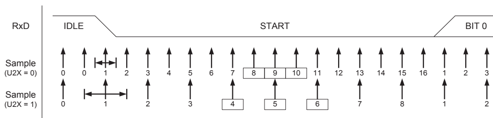
Figure 83. Start Bit Sampling
