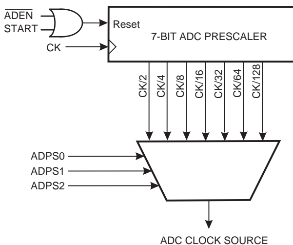
Figure 110. ADC Prescaler
