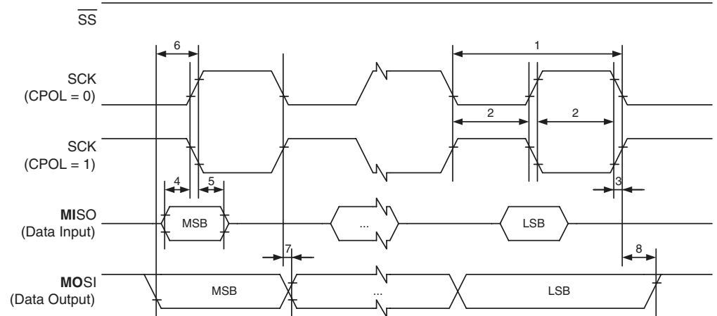
Figure 136. SPI Interface Timing Requirements (Master Mode)
