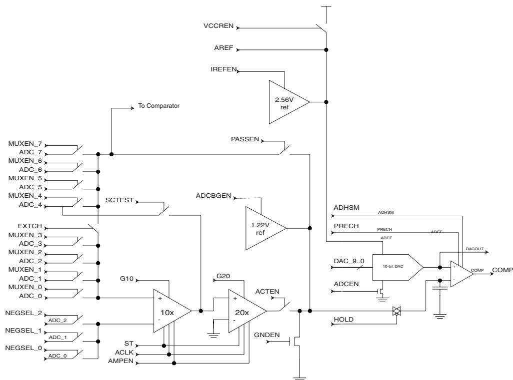
Figure 114. Analog to Digital Converter
