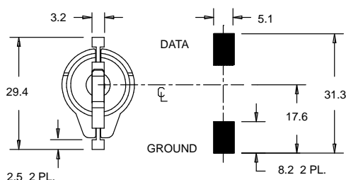
DS9094FS RECOMMENDED PAD SIZE
