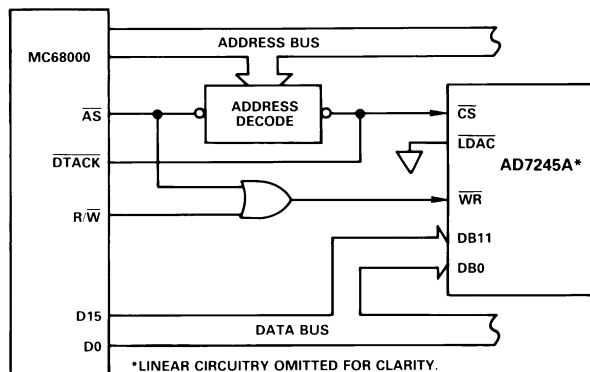
Figure 14. AD7245A to 68000 Interface
