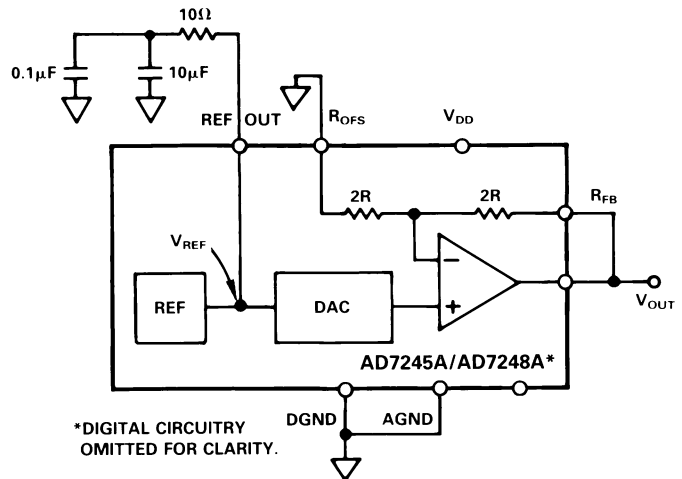
Figure 8. Unipolar (0 to +10 V) Configuration
