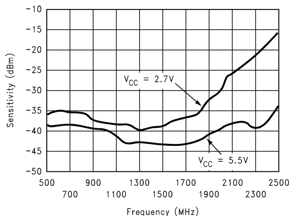
LMX2371 RF Input Sensitivity vs Frequency
