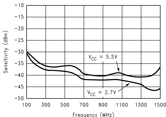
LMX2372 RF Sensitivity vs Frequency
