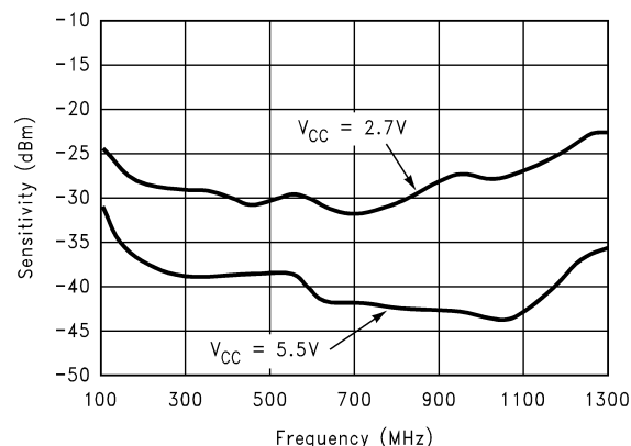
Auxiliary Input Sensitivity vs Frequency
