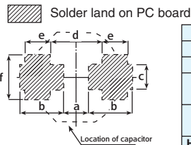
Fig.3 Resin-Molded chip type <Share with Ta/Al multilayer capacitors (7343 size)>
