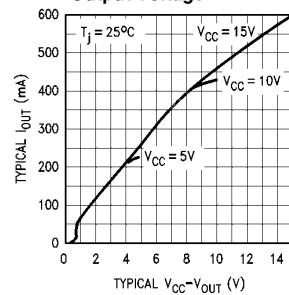
Typical Source Current vs Output Voltage
