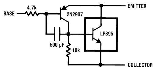
Composite PNP
