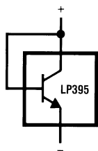
Two Terminal Current Limiter
