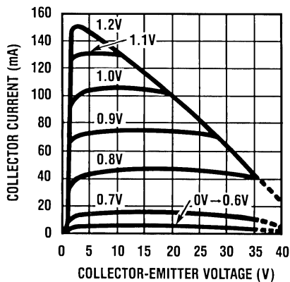
Collector Characteristics
