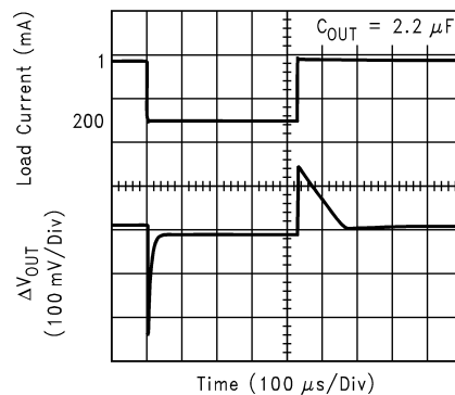
LDO2 (2.85V Option) Load Transient
