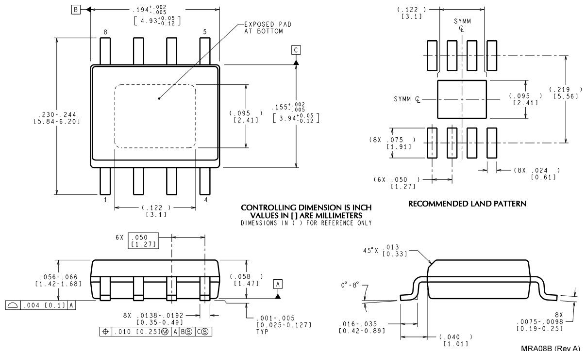
PSOP-8 8-Lead Molded PSOP-2 NS Package Number MRA08B
