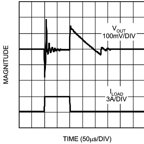
Load Transient Response (Both Oscon 10\mu\text{F}/3\text{A} )
