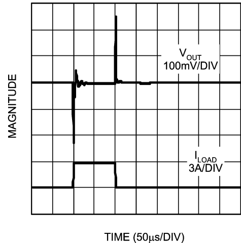
Load Transient Response (SANYO 150\mu\text{F}/3\text{A} )
