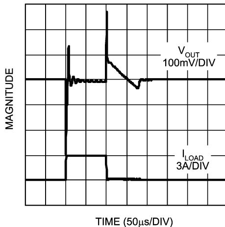
Load Transient Response (Tantalum 10\mu\text{F}/3\text{A} )
