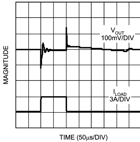
Load Transient Response (Both POSCAP 100\mu\text{F}/3\text{A} )
