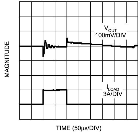
Load Transient Response (Both Oscon 100\mu\text{F}/3\text{A} )
