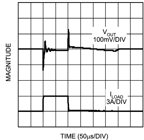
Load Transient Response (Tantalum 100\mu\text{F}/3\text{A} )
