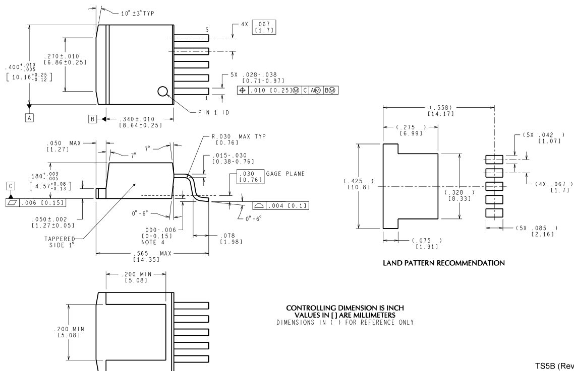
Molded PSOP-2, 8 Lead Package (PSOP-8) NS Package Number MRA08A
