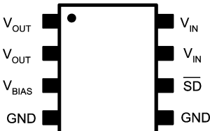
PSOP-8, Top View
