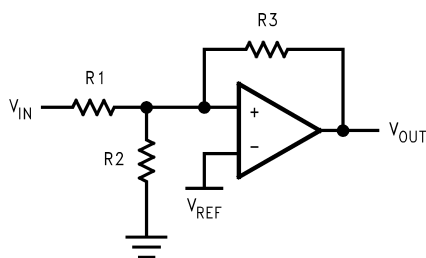
FIGURE 2. Additional Hysteresis
