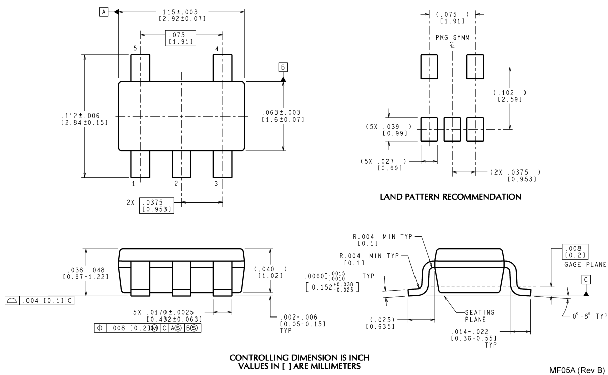
5-Pin SOT23-5 Tape and Reel NS Package Number MF05A
