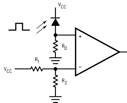
FIGURE 6. IR Receiver
