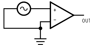
FIGURE 3. Zero-Crossing Detector
