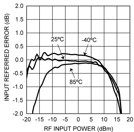
Input Referred Error vs. RF Input Power @ 1800 MHz
