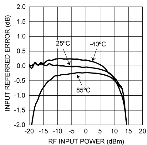
Input Referred Error vs. RF Input Power @ 900 MHz
