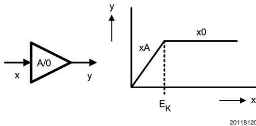
FIGURE 7. Gain Cell
