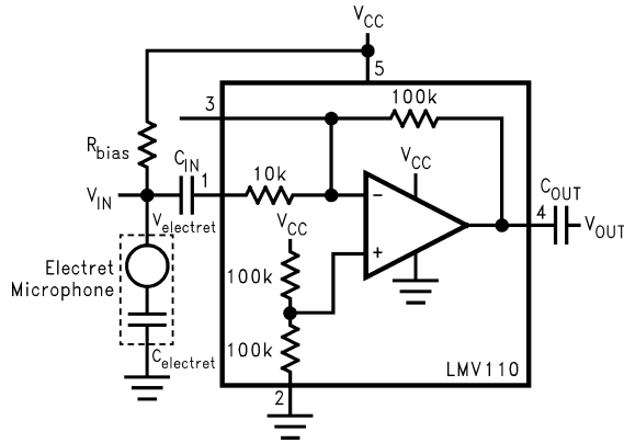
FIGURE 5. Microphone Preamplifier with 20dB Gain
