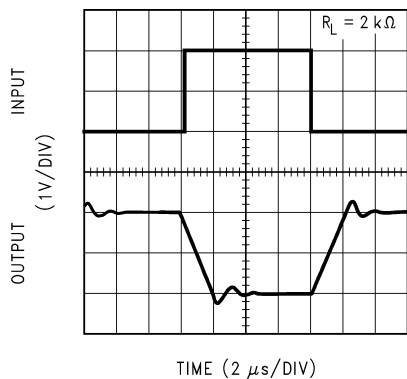
Inverting Large Signal Pulse Response LMV101
