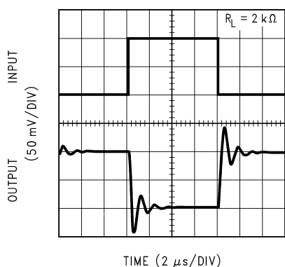
Inverting Small Signal Pulse Response LMV101
