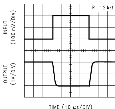
Inverting Large Signal Pulse Response LMV110
