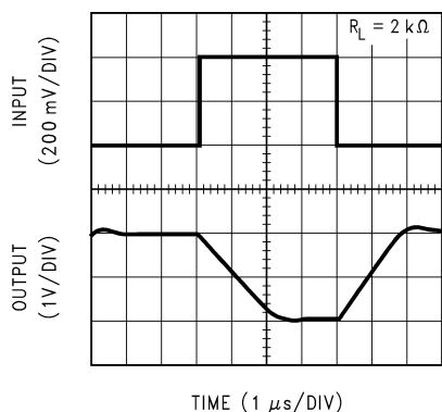
Inverting Large Signal Pulse Response LMV105
