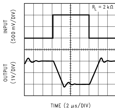
Inverting Large Signal Pulse Response LMV102
