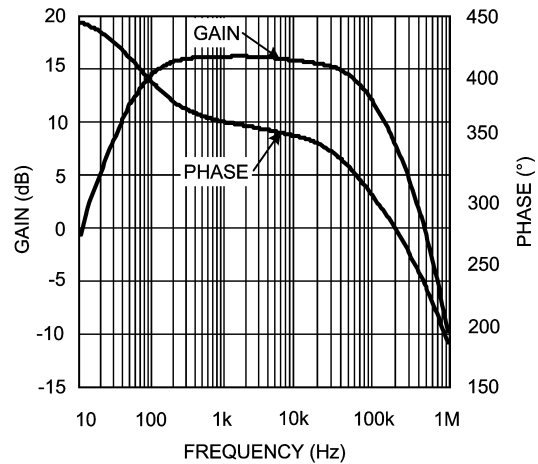
FIGURE 5. Gain vs. Frequency
