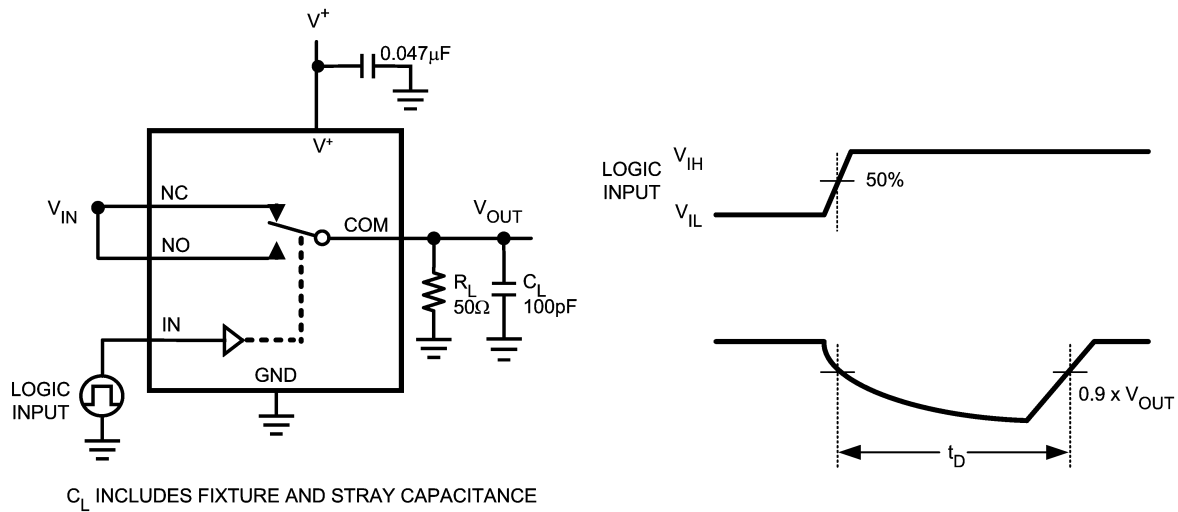
FIGURE 2. Break-Before Make Delay
