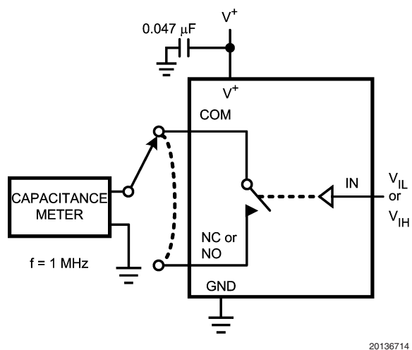
FIGURE 4. Channel Capacitance
