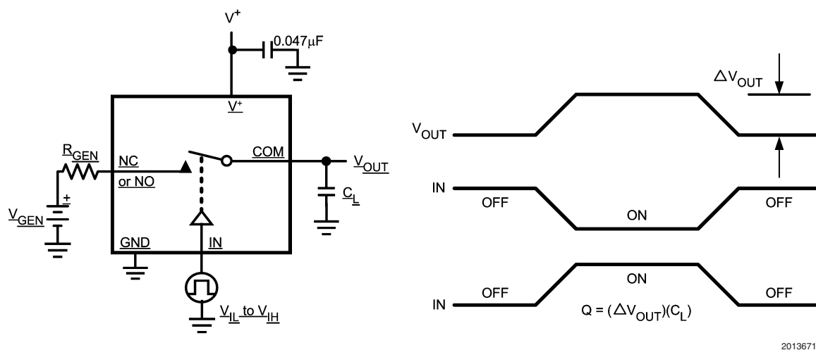
FIGURE 3. Charge Injection
