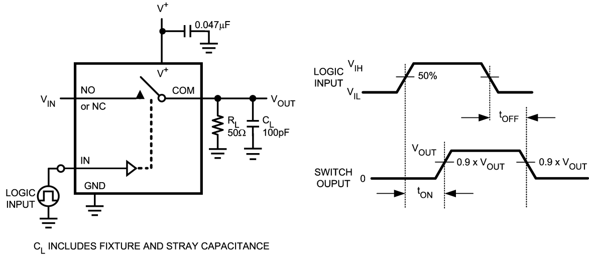
FIGURE 1. t_{ON} / t_{OFF} Time
