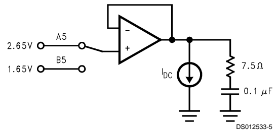
FIGURE 4. 13 mA Sink/Source
