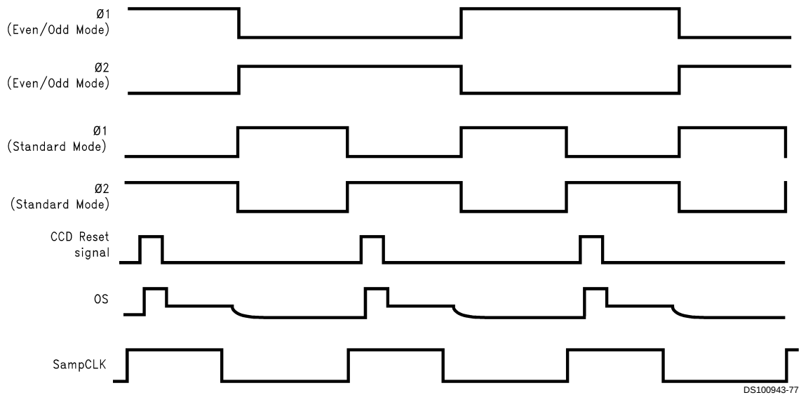
FIGURE 5. CDS Timing
