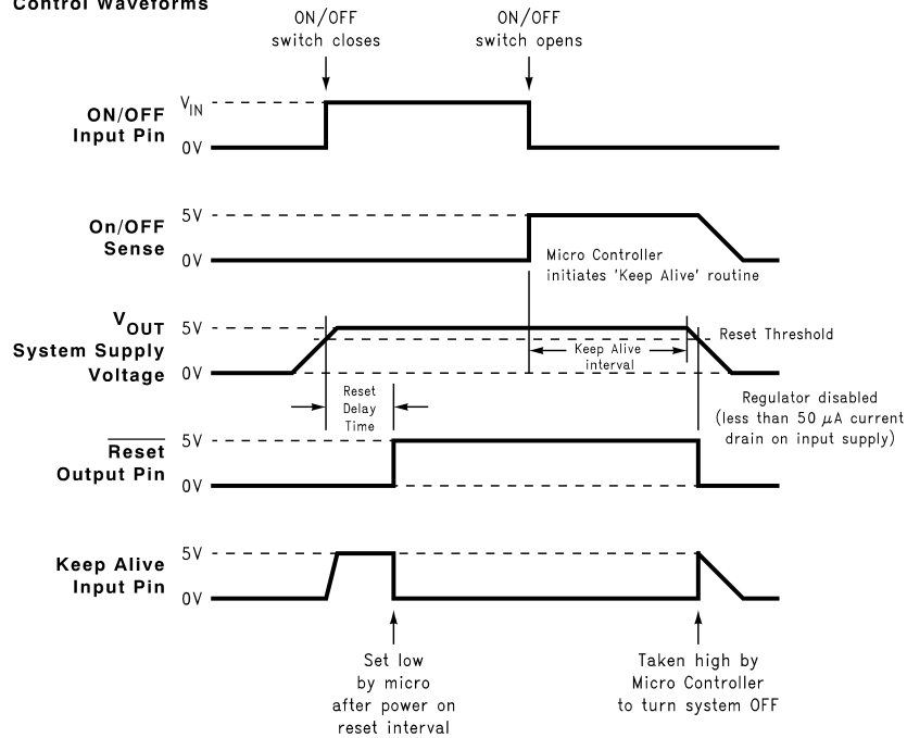
Control Waveforms
