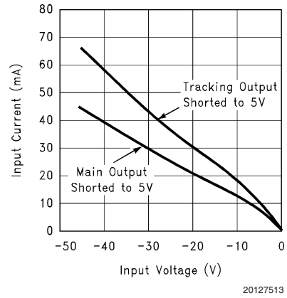
Reverse Battery Input Current
