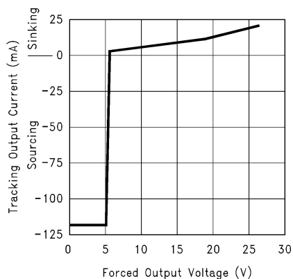
Tracking Output Short Circuit Current
