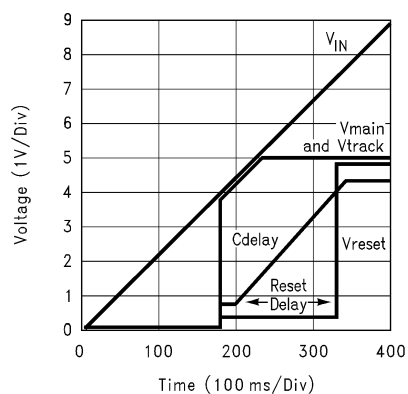
Turn-ON Characteristic
