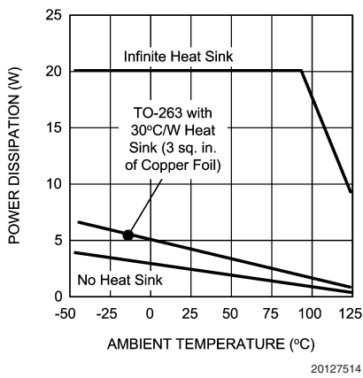
Maximum Power Dissipation
