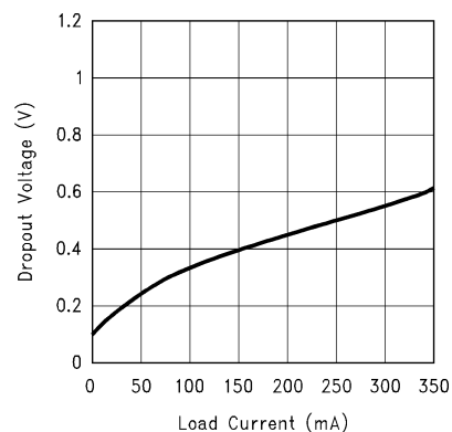
Main Regulator Dropout Voltage vs Load Current
