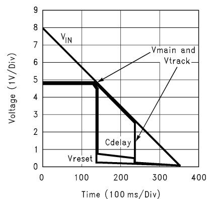
Turn-OFF Characteristic
