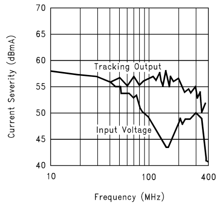
BCI Susceptibility Modulation 2 (1 kHz, 80% AM modulation)
