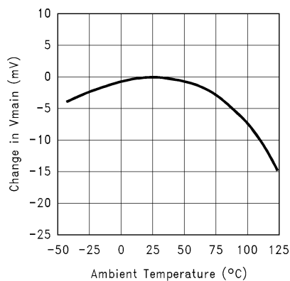
Normalized Main Output Voltage vs Temperature
