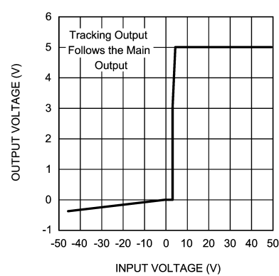
Main Output Voltage at Input Voltage Extremes
