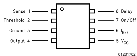
Top View Order Number LM9061N See NS Package Number N08E
