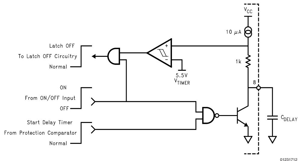
FIGURE 4. Delay Timer
