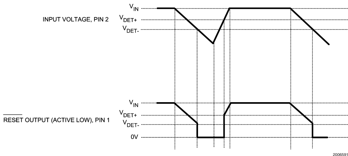
FIGURE 2. Timing Waveforms
