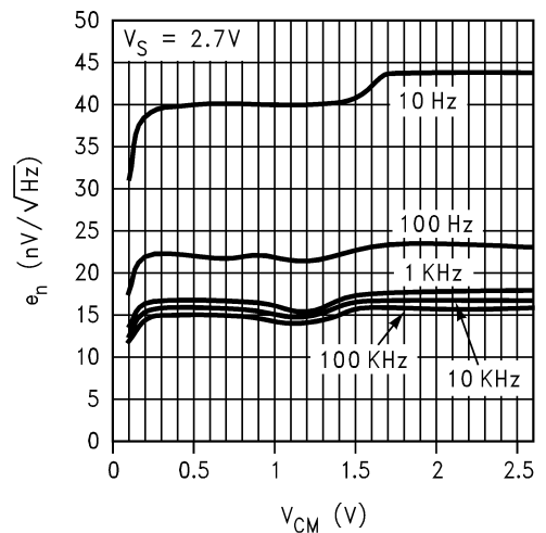
Input Noise Voltage vs. V_{CM}
