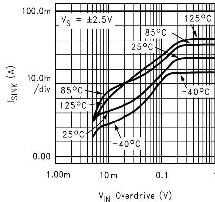
FIGURE 4. Output Short Circuit Sinking Current vs. Input Overdrive
