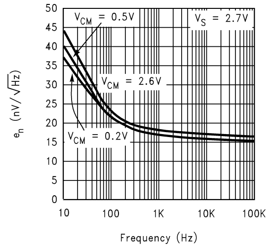
Input Noise Voltage for Various V_{CM}
