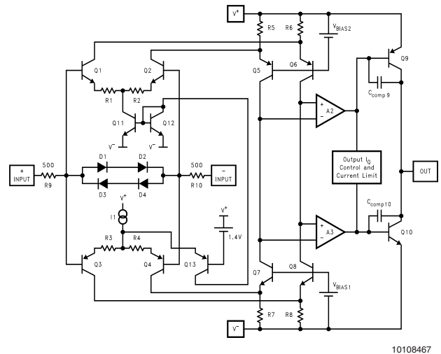
FIGURE 1. Simplified schematic Diagram
