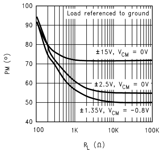
Phase Margin vs. Load
