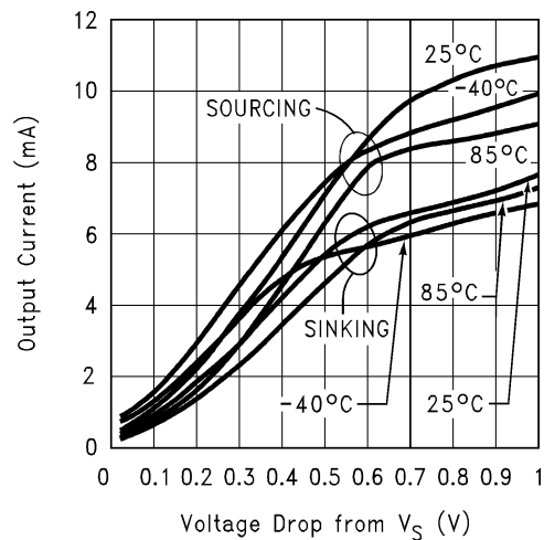
V_O vs I_O , V_S = \pm 1.1\text{V}
