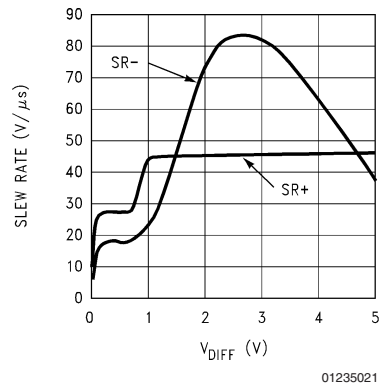
FIGURE 2. Slew Rate vs. V DIFF
