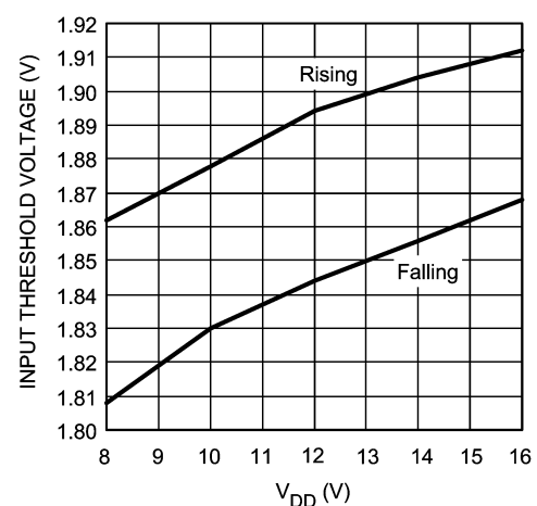
Input Thresholds vs Supply Voltage
