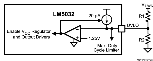
FIGURE 23. UVLO Circuit
