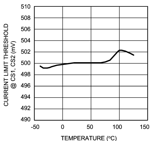
FIGURE 14. Current Limit Threshold at CS1, CS2 vs. Temperature
