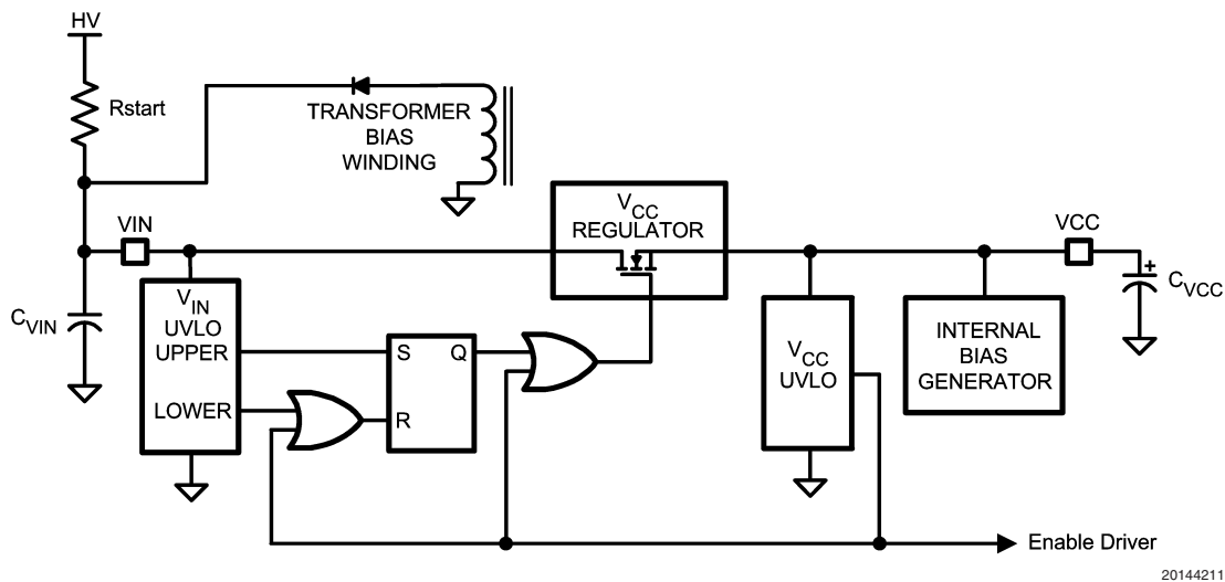
FIGURE 2. Start-Up Circuit Block Diagram
