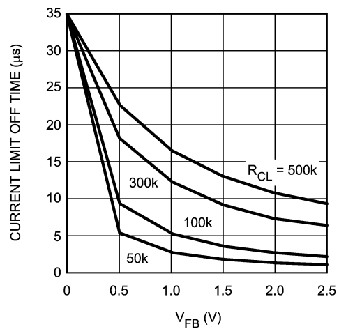
FIGURE 5. Current Limit Off-Time vs V_{FB} and R_{CL}
