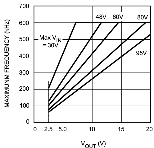
FIGURE 4. Maximum Frequency vs V_{OUT} and V_{IN}
