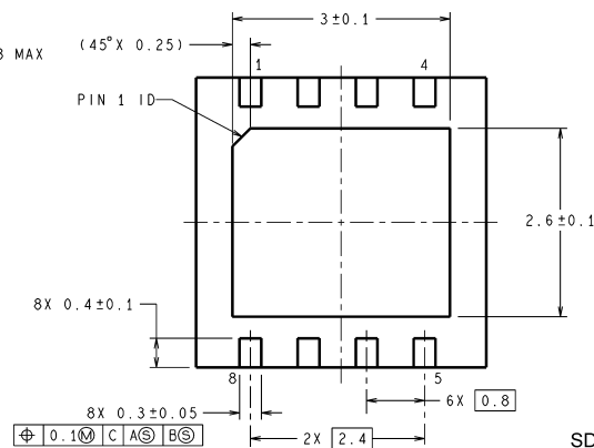
8-Lead LLP Package NS Package Number SDC08A
