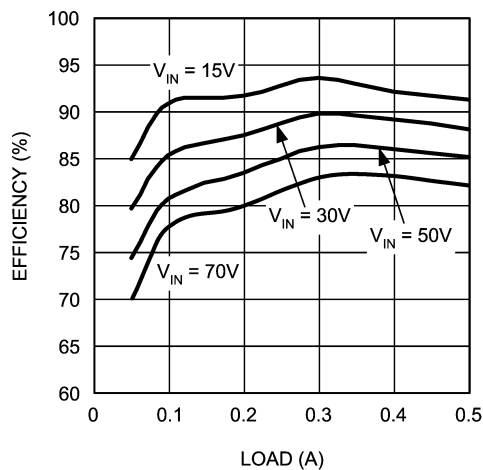
LM5007EP 10V Output Efficiency
