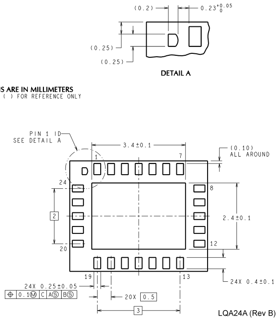
24-Lead Molded pkg, Leadframe Package LLP Order Number LM4863LQ NS Package Number LQA24A
