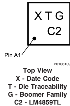
micro SMD Marking
