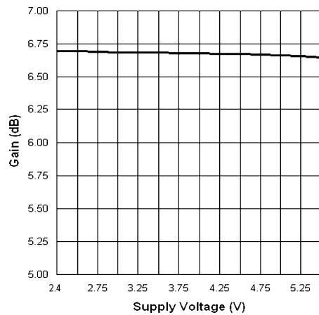
Gain vs Supply Voltage R_{in} = 150k\Omega
