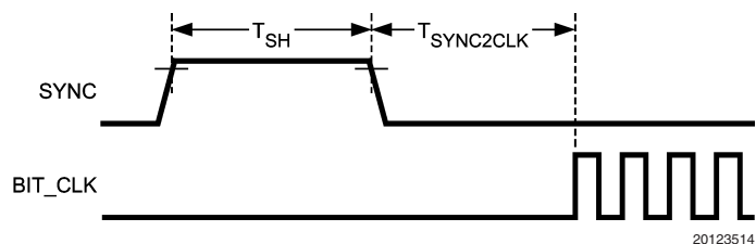
Warm Reset
