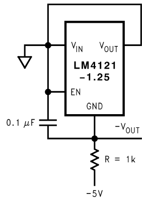
Voltage Reference with Negative Output
