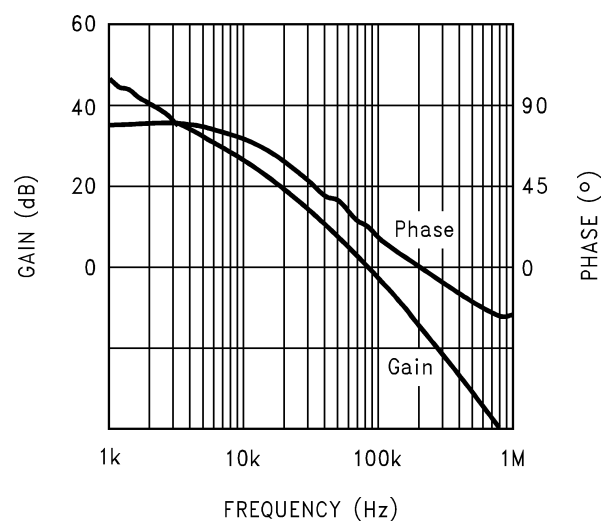
Bode Plot
