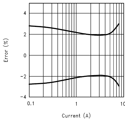
Error vs Current (LM3812-7.0 and LM3813-7.0) (Note 10)
