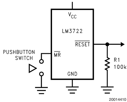
FIGURE 1. Circuit for \overline{\text{RESET}} Valid from V_{CC} = 0V
