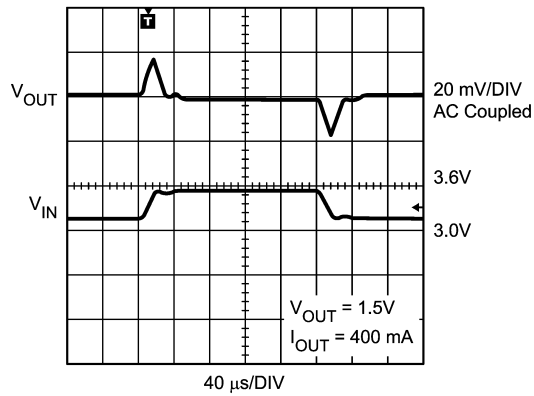
Line Transient Response (PWM Mode)
