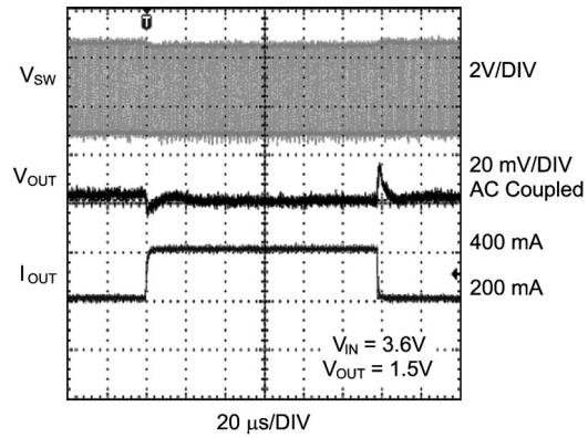
Load Transient Response (PWM Mode)
