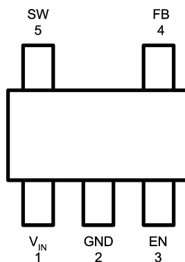
FIGURE 3. TopView SOT23-5 Package NS Package Number MF05A
