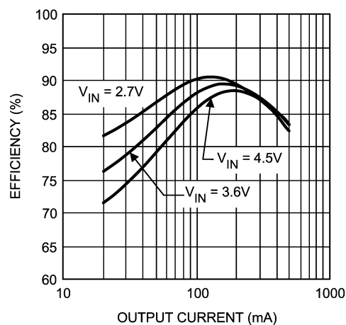
Efficiency vs. Output Current (SYNC/MODE = V_{IN} , V_{OUT} = 1.05V )
